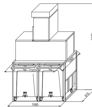
ROLLER BIN 280 - SPLIT 750/1300
