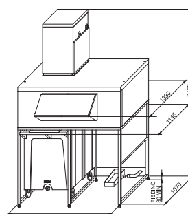
DOUBLE ROLLER BIN 1100 - GM 2000 SPLIT
