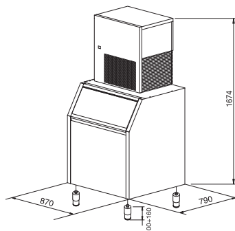
BIN T 420 - GM 550 / GM 1100 GM 1100 SPLIT - MGT 290/900
