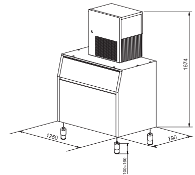
BIN T 830 - GM 550 - GM 1100 GM 1100 Split - MGT 290/900
