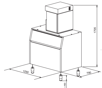
BIN T 830 - Split 750 - Split 1300
