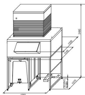
DOUBLE ROLLER BIN 1100 - GM 2000
