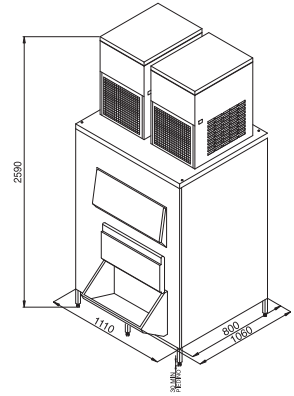
BIN 1200 DD - Double GM1100 Double GM 1100 SPLIT - Double MGT 900
