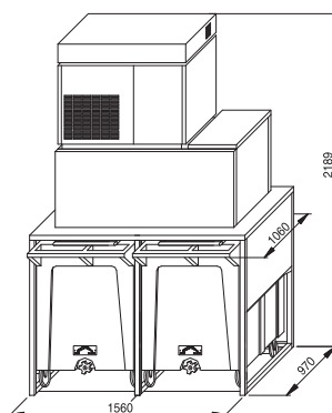
ROLLER BIN 280 - SM 750/1300
