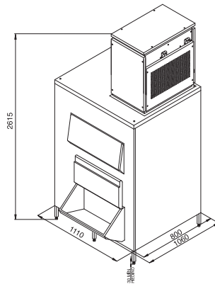
BIN 1200 DD - GM 2000 SPLIT
