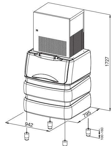
BIN PE530 - GM 550 / GM 1100 GM 1100 SPLIT - MGT 290/900
