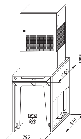
ROLLER BIN 140 - GM 550 / GM 1100 GM 1100 SPLIT - MGT 290/900
