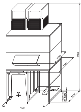
DRB 2500 - Double GM 1100/1100 SPLIT Double MGT 900
