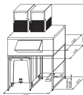
DOUBLE ROLLER BIN 1100 DOUBLE GM 550 / DOUBLE GM 1100 DOUBLE GM 1100 SPLIT - DOUBLE MGT900
