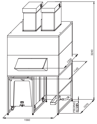
DRB 2500 - Double SPLIT 1300
