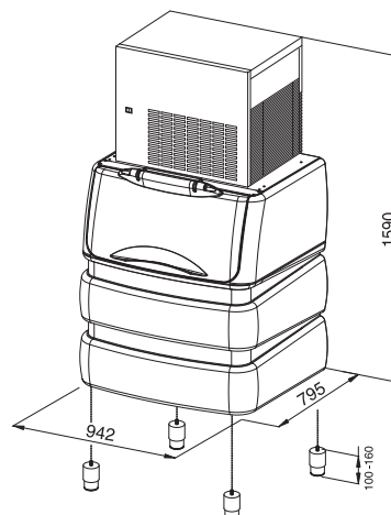
BIN PE530 - GM 330
