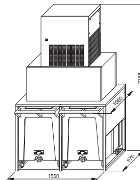
ROLLER BIN 280 - GM 550/1100 GM 1100 SPLIT - MGT 290/900
