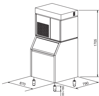
BIN T 420 - SM 750
